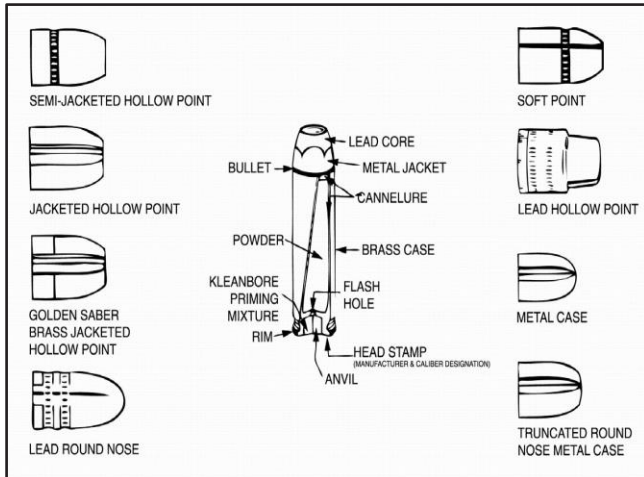
(Figure 3-5) Handgun bullet styles
